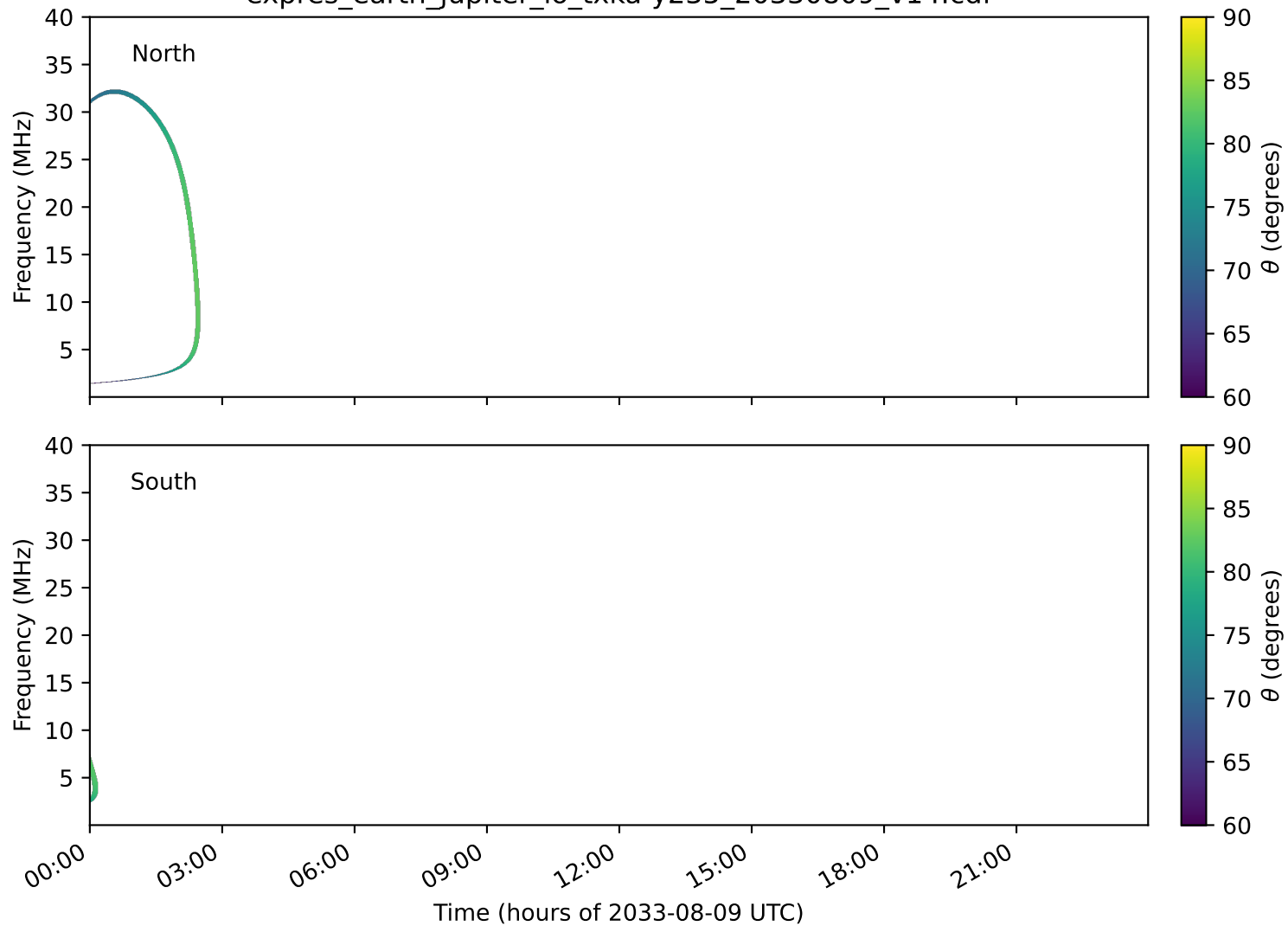
expres_earth_jupiter_io_txka-y235_20330809_v14.cdf
