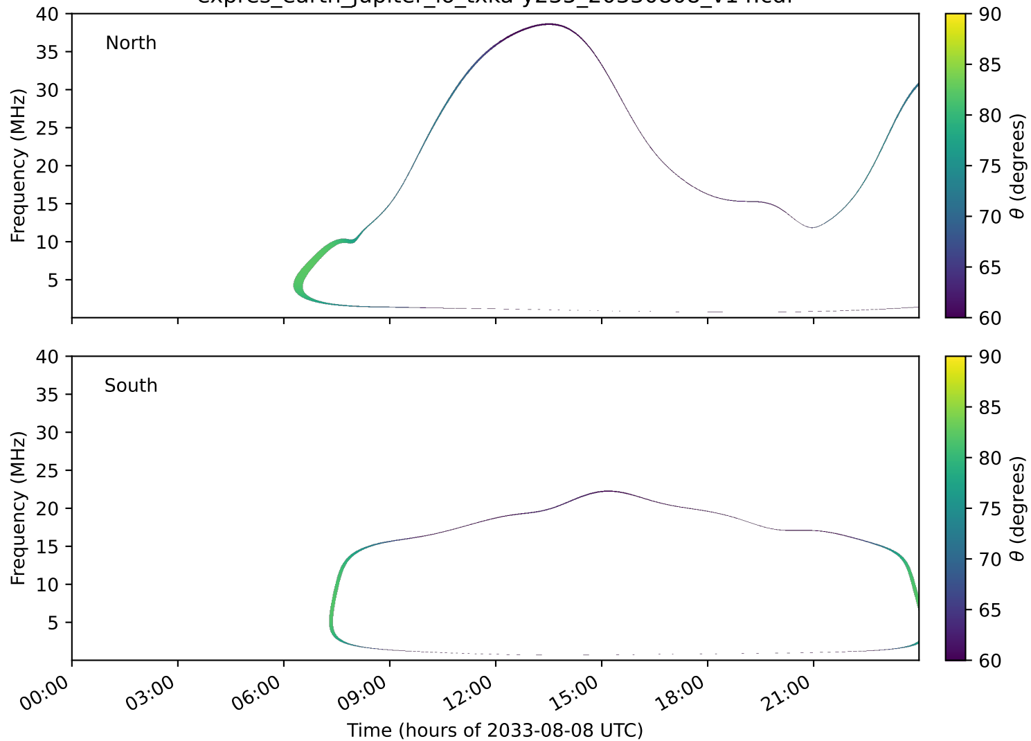
expres_earth_jupiter_io_txka-y235_20330808_v14.cdf
