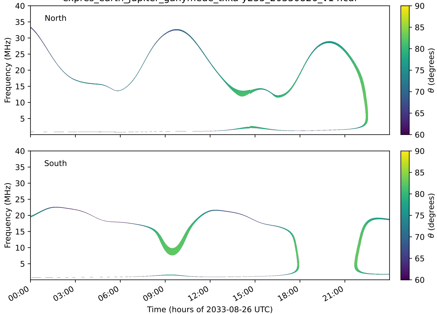
expres_earth_jupiter_ganymede_txka-y235_20330826_v14.cdf
