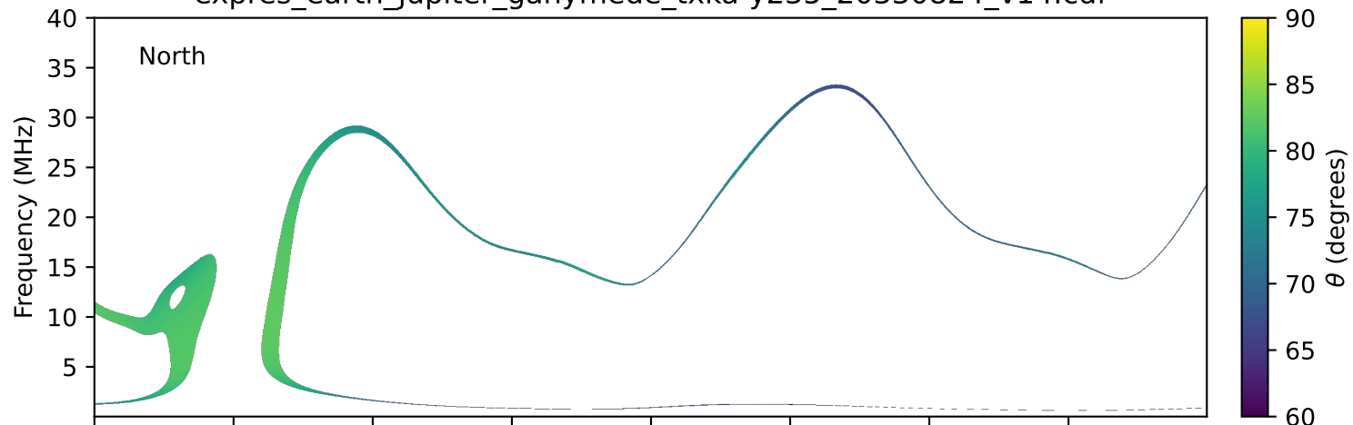
expres_earth_jupiter_ganymede_txka-y235_20330824_v14.cdf
