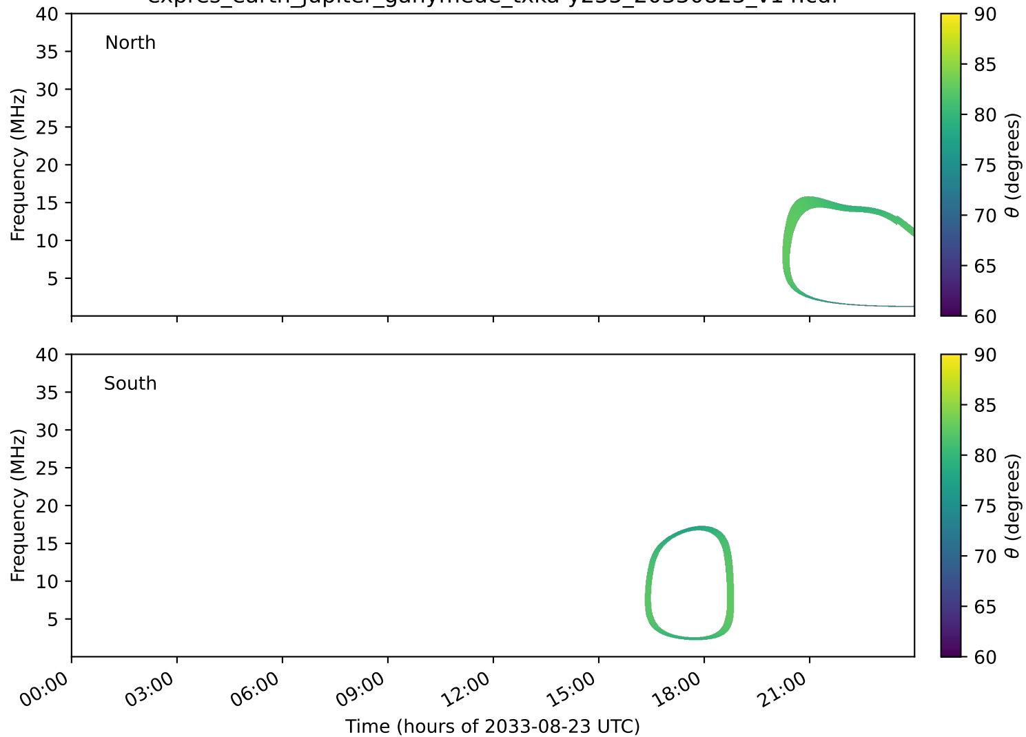
expres_earth_jupiter_ganymede_txka-y235_20330823_v14.cdf
