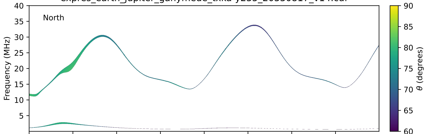
expres_earth_jupiter_ganymede_txka-y235_20330817_v14.cdf
