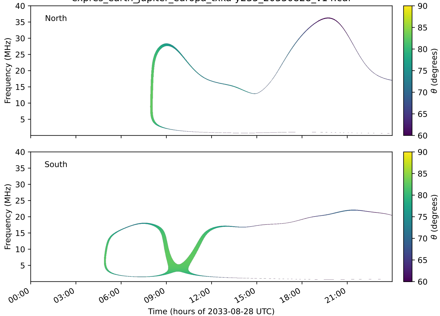
expres_earth_jupiter_europa_txka-y235_20330828_v14.cdf
