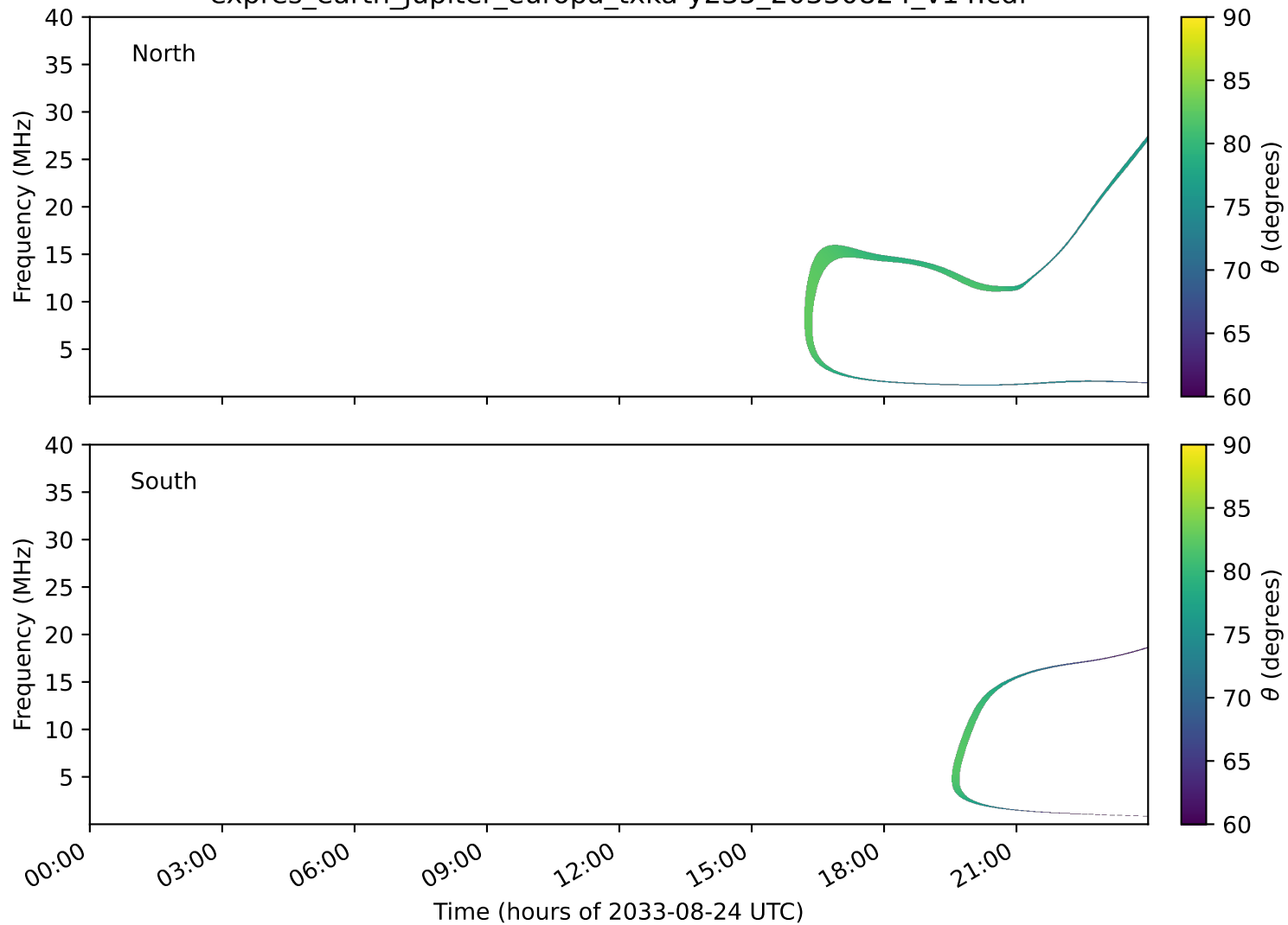
expres_earth_jupiter_europa_txka-y235_20330824_v14.cdf
