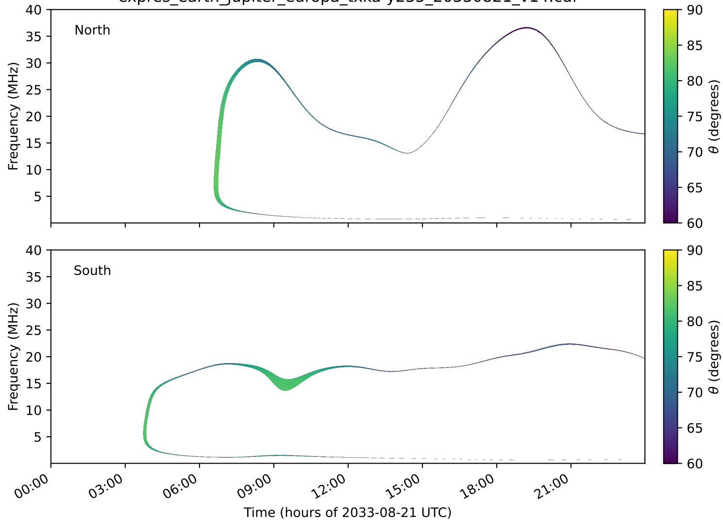
expres_earth_jupiter_europa_txka-y235_20330821_v14.cdf
