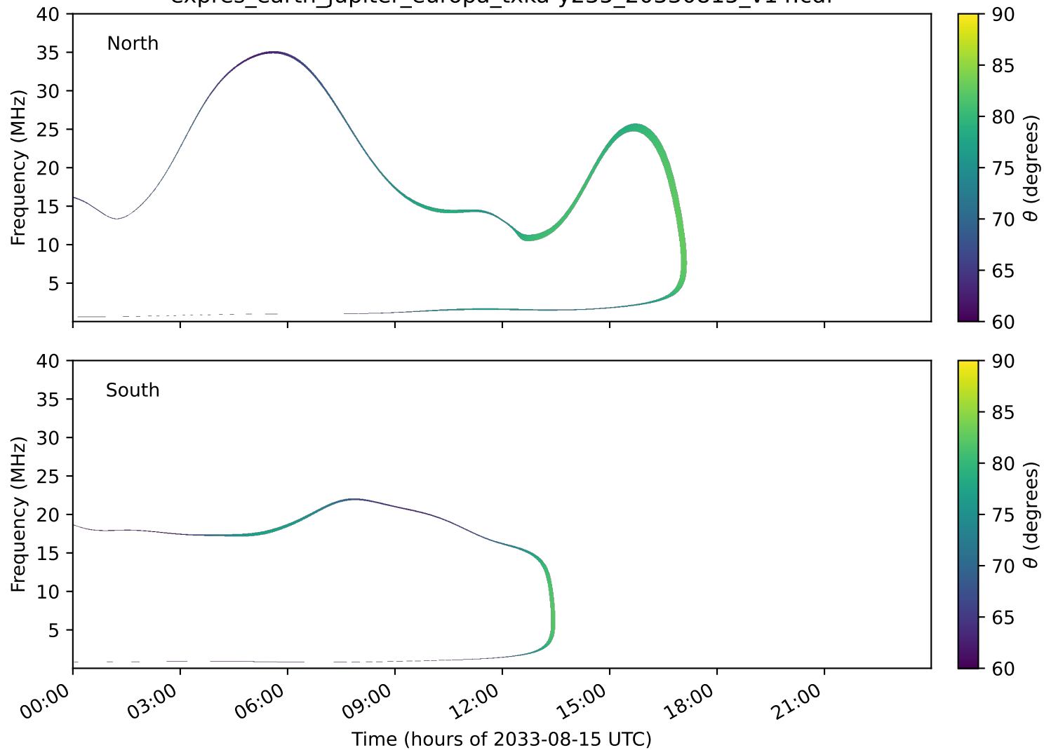
expres_earth_jupiter_europa_txka-y235_20330815_v14.cdf
