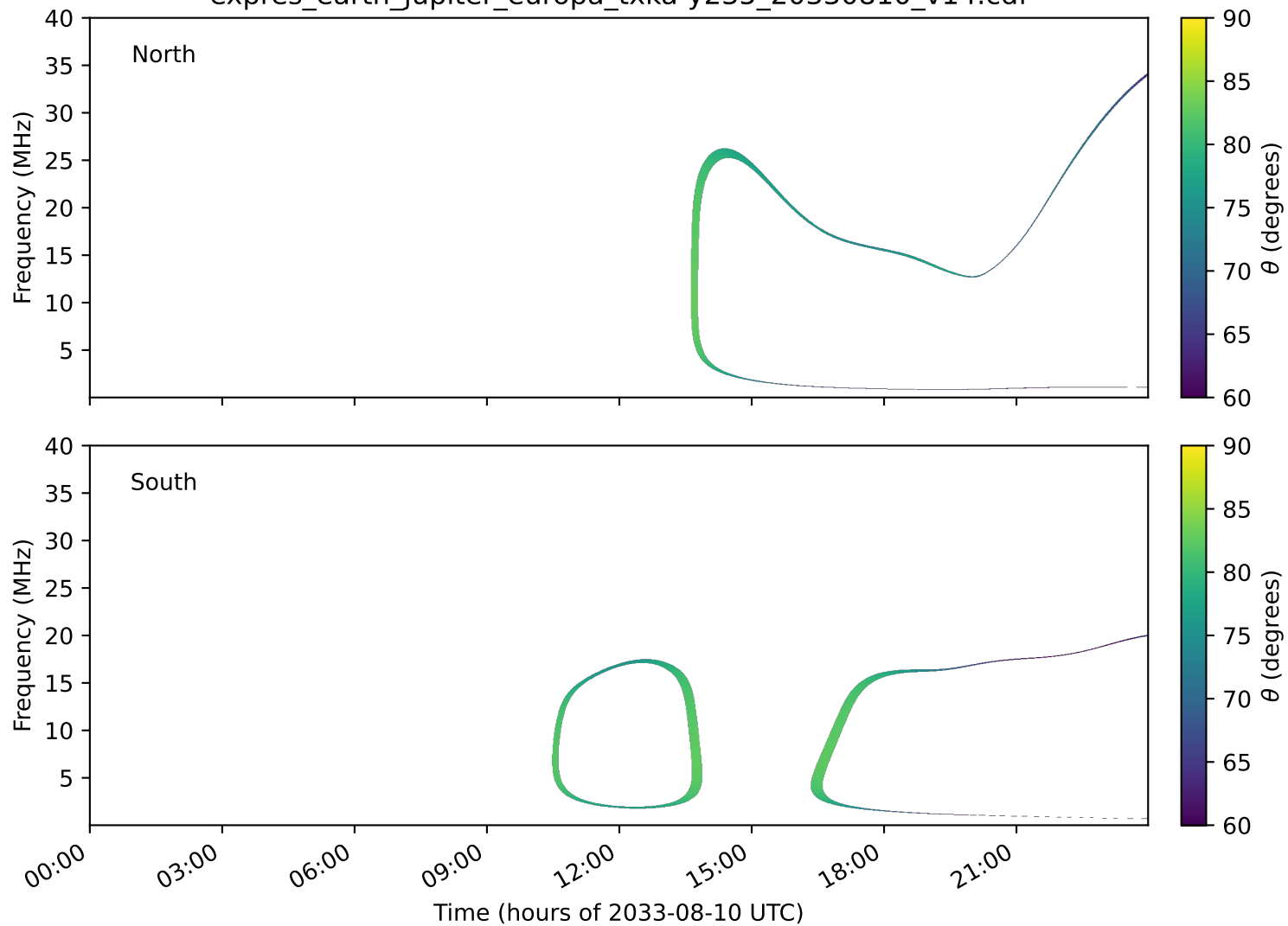
expres_earth_jupiter_europa_txka-y235_20330810_v14.cdf
