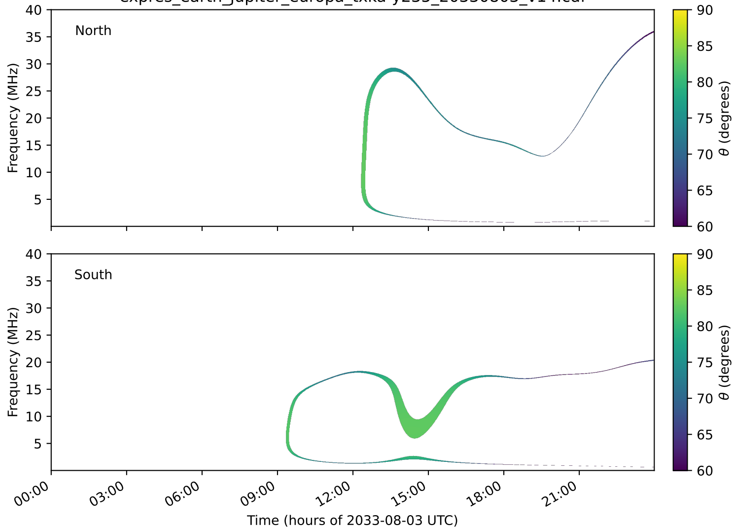
expres_earth_jupiter_europa_txka-y235_20330803_v14.cdf
