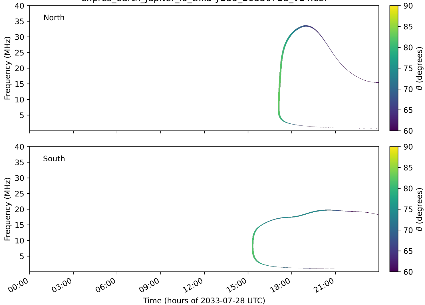
expres_earth_jupiter_io_txka-y235_20330728_v14.cdf
