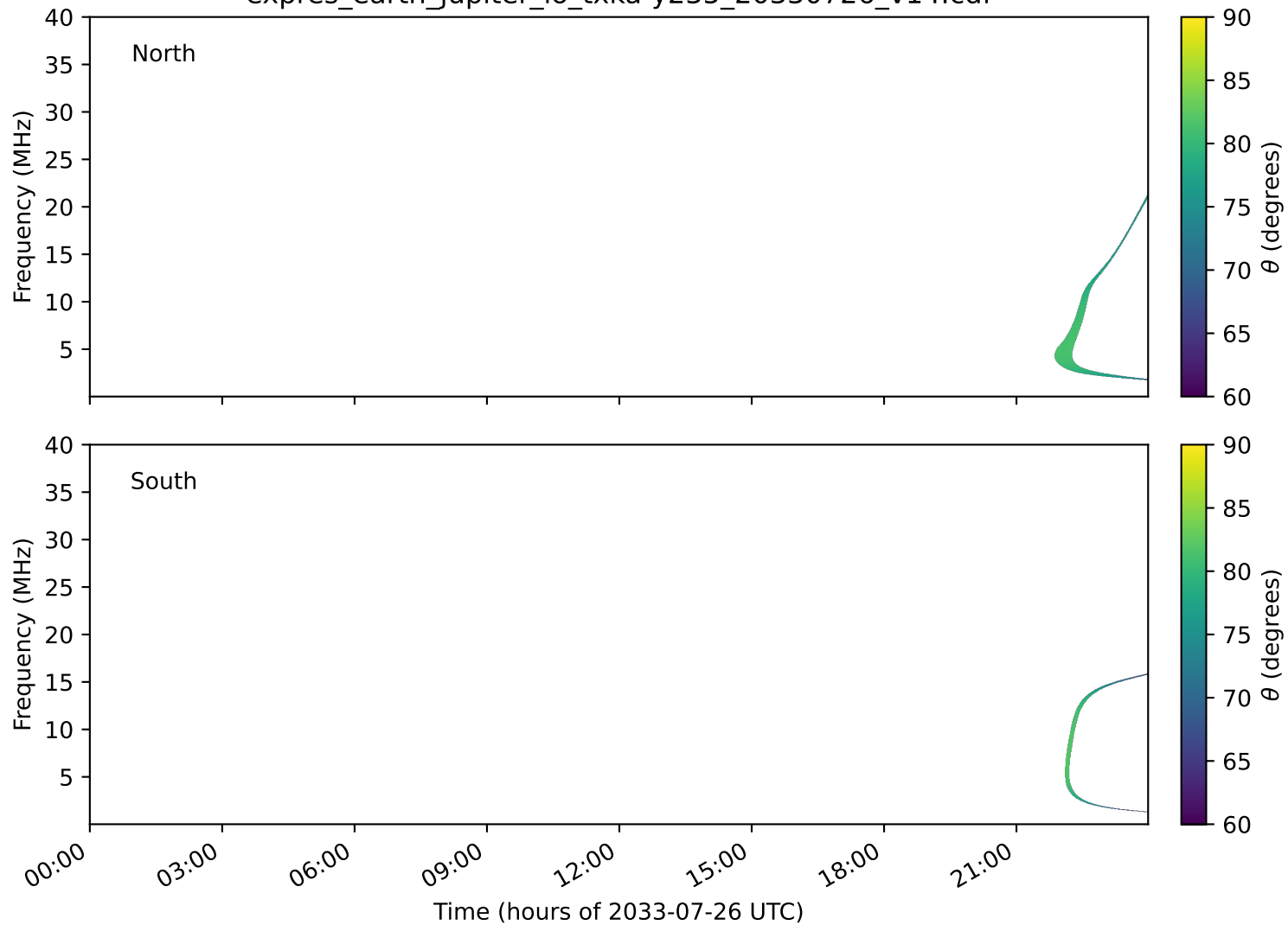
expres_earth_jupiter_io_txka-y235_20330726_v14.cdf
