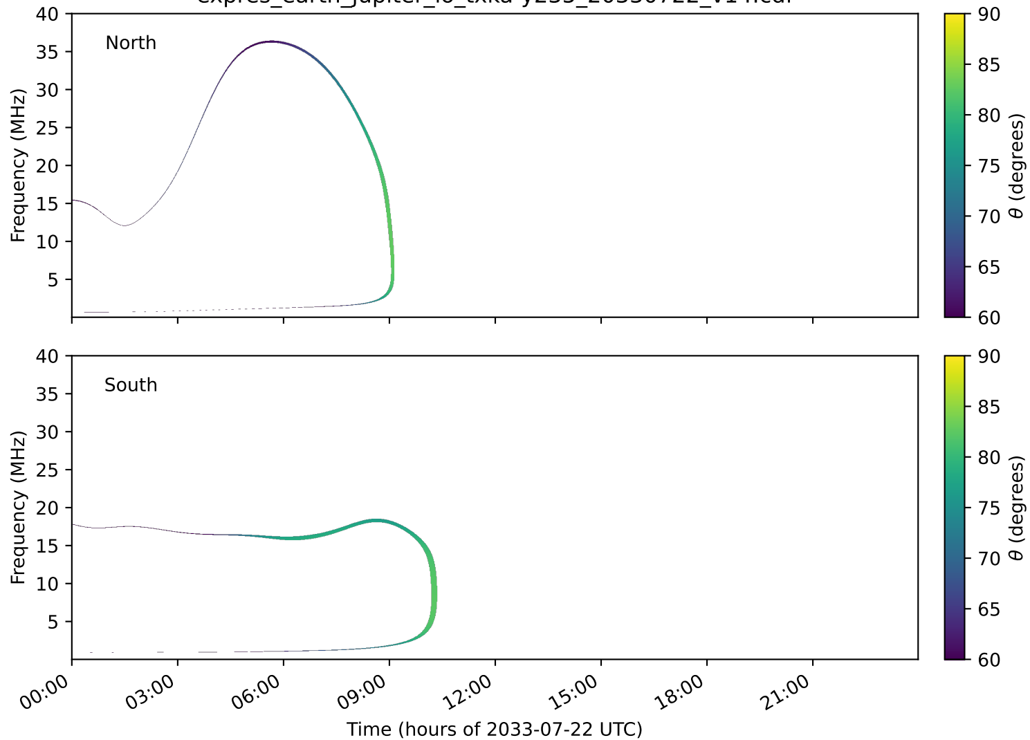
expres_earth_jupiter_io_txka-y235_20330722_v14.cdf
