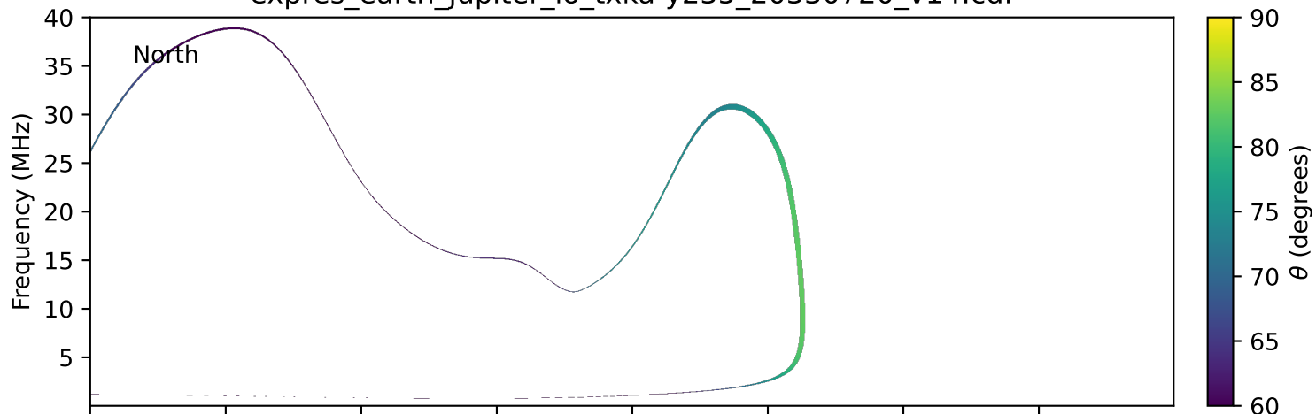
expres_earth_jupiter_io_txka-y235_20330720_v14.cdf
