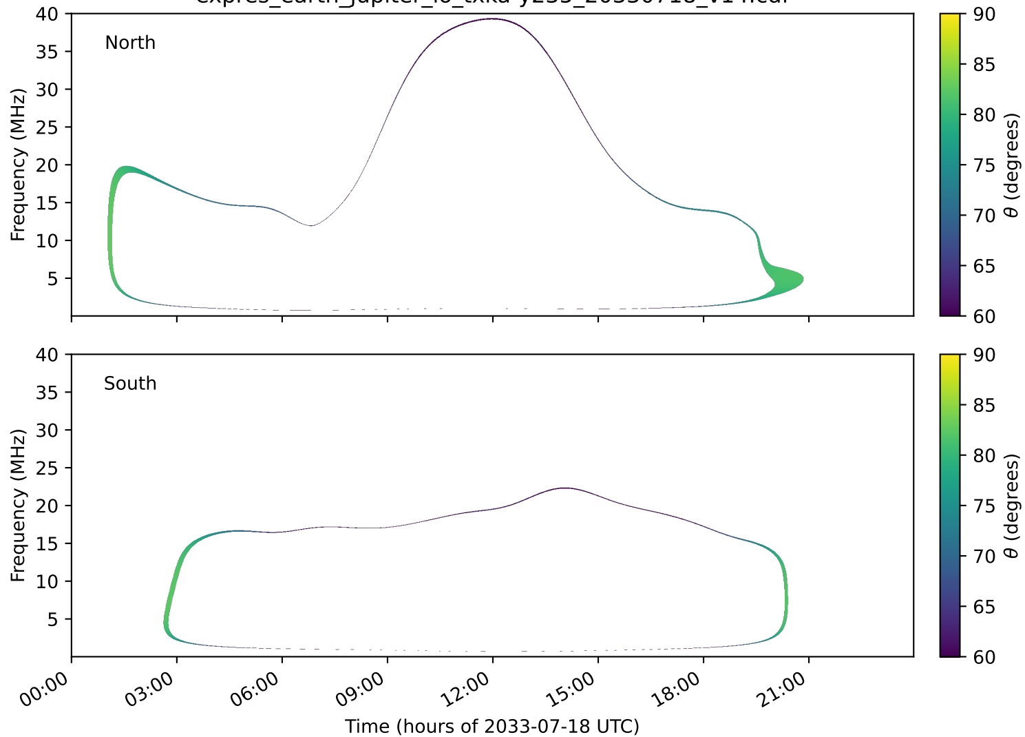
expres_earth_jupiter_io_txka-y235_20330718_v14.cdf
