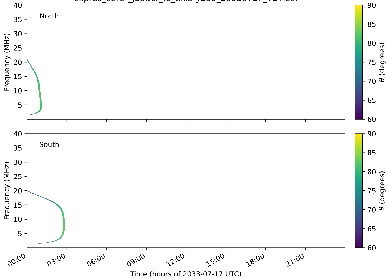
expres_earth_jupiter_io_txka-y235_20330717_v14.cdf
