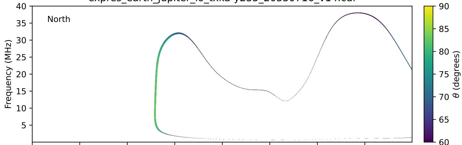
expres_earth_jupiter_io_txka-y235_20330716_v14.cdf
