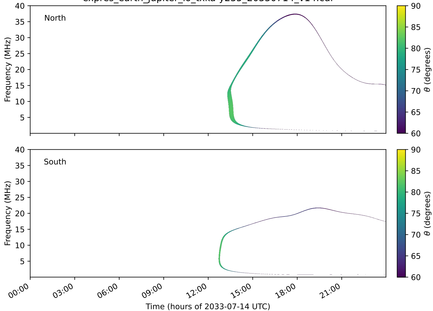
expres_earth_jupiter_io_txka-y235_20330714_v14.cdf
