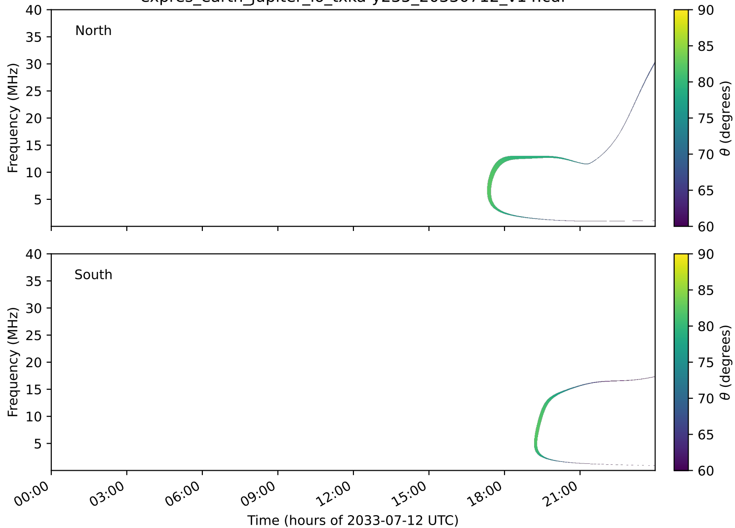
expres_earth_jupiter_io_txka-y235_20330712_v14.cdf
