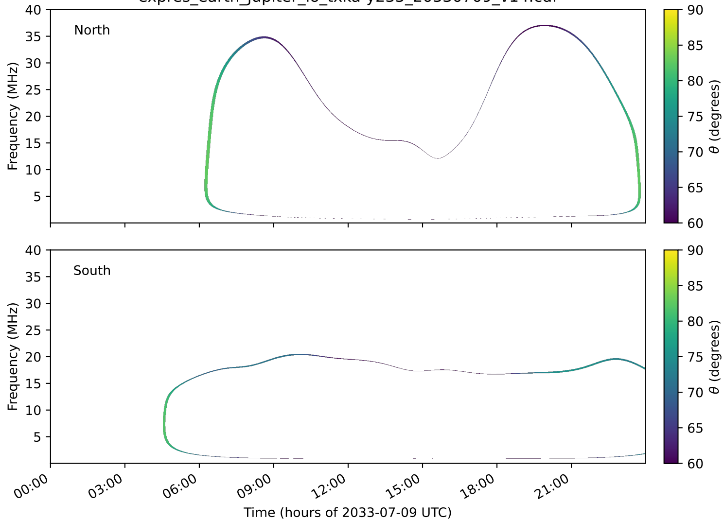
expres_earth_jupiter_io_txka-y235_20330709_v14.cdf
