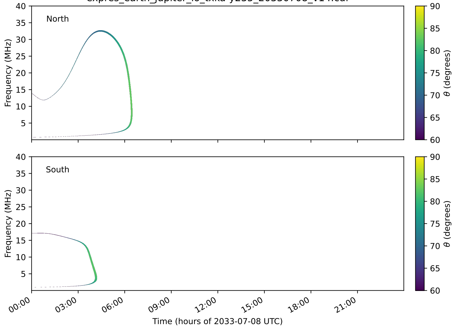
expres_earth_jupiter_io_txka-y235_20330708_v14.cdf
