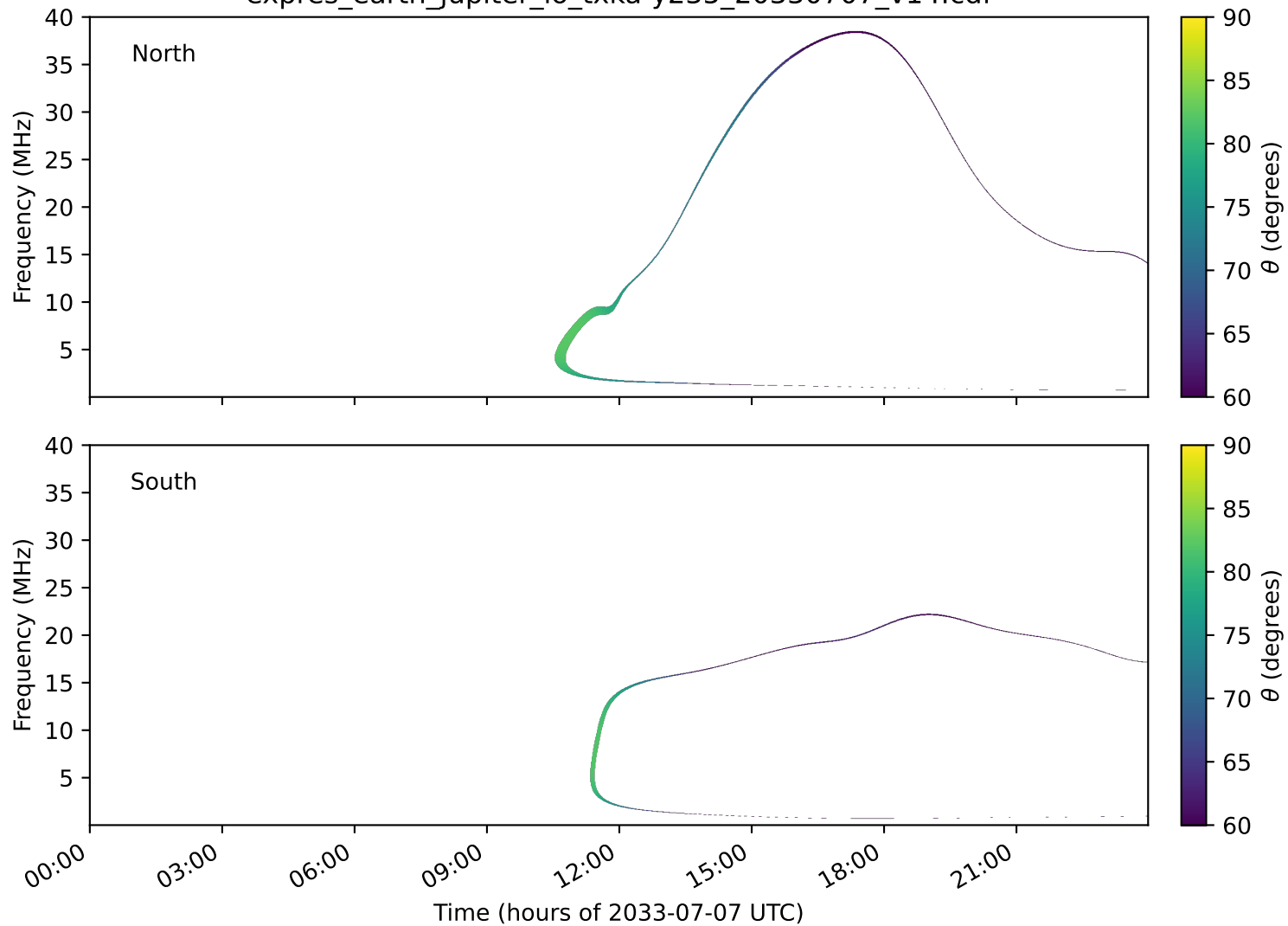
expres_earth_jupiter_io_txka-y235_20330707_v14.cdf
