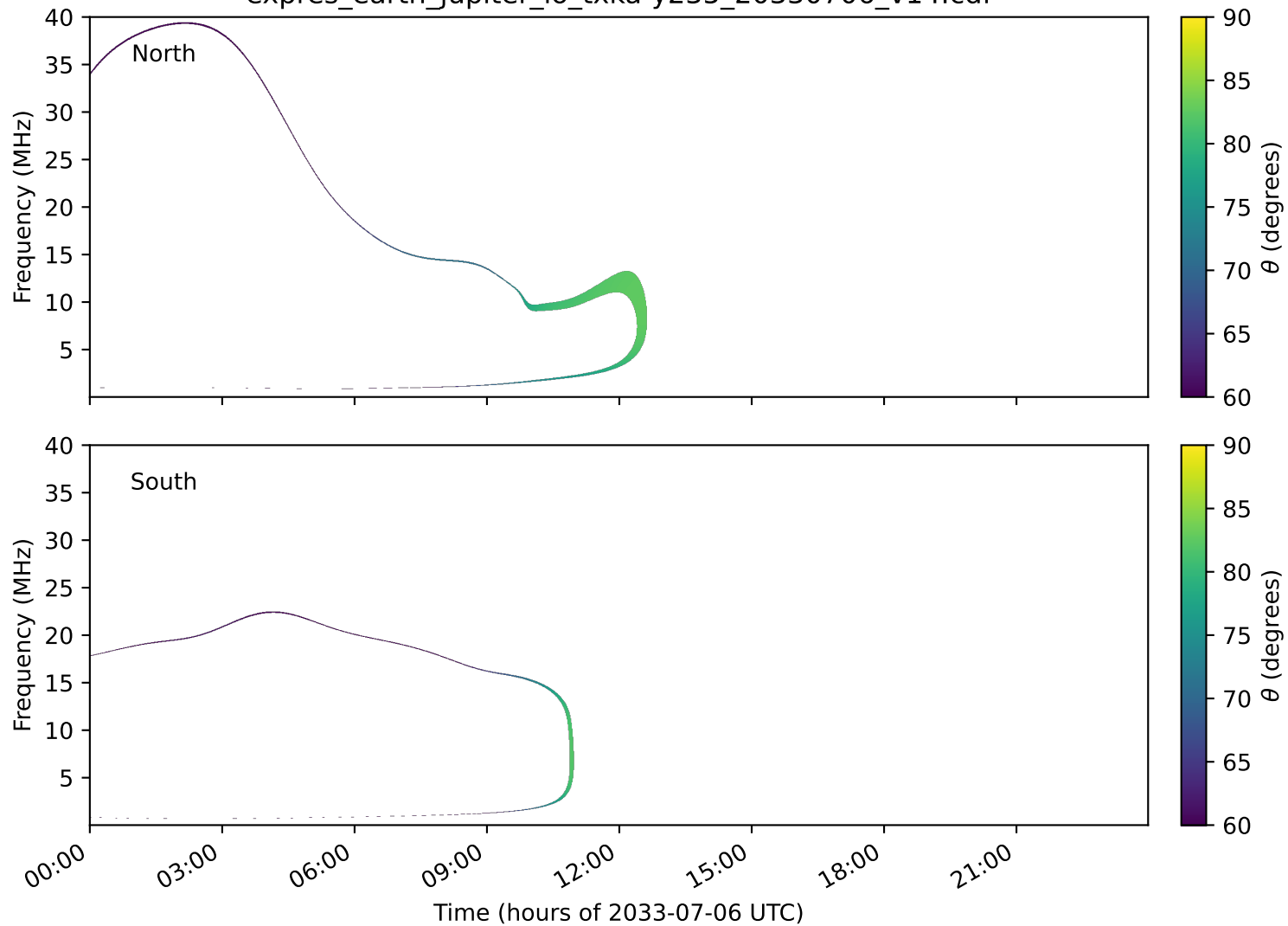
expres_earth_jupiter_io_txka-y235_20330706_v14.cdf
