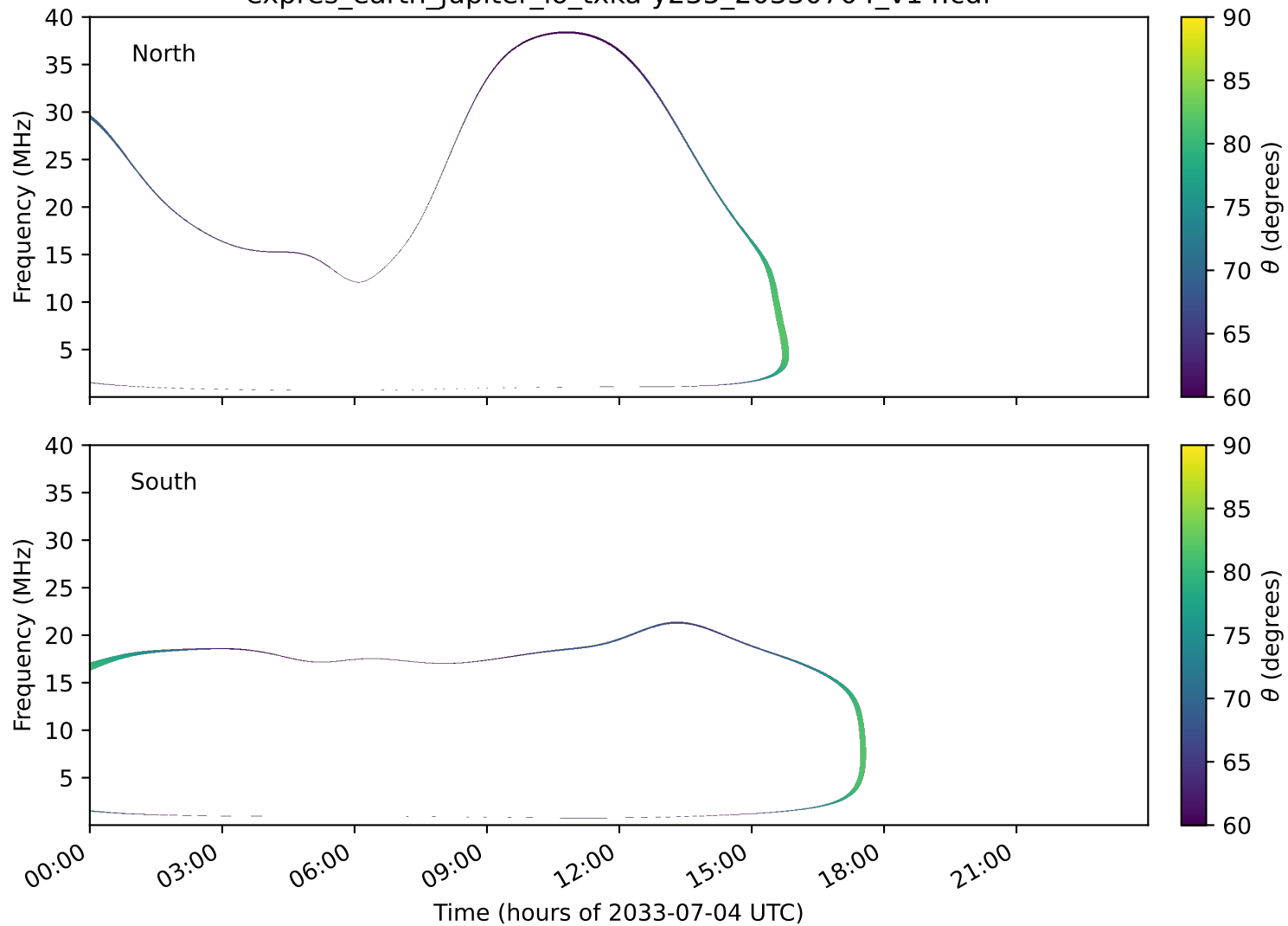
expres_earth_jupiter_io_txka-y235_20330704_v14.cdf
