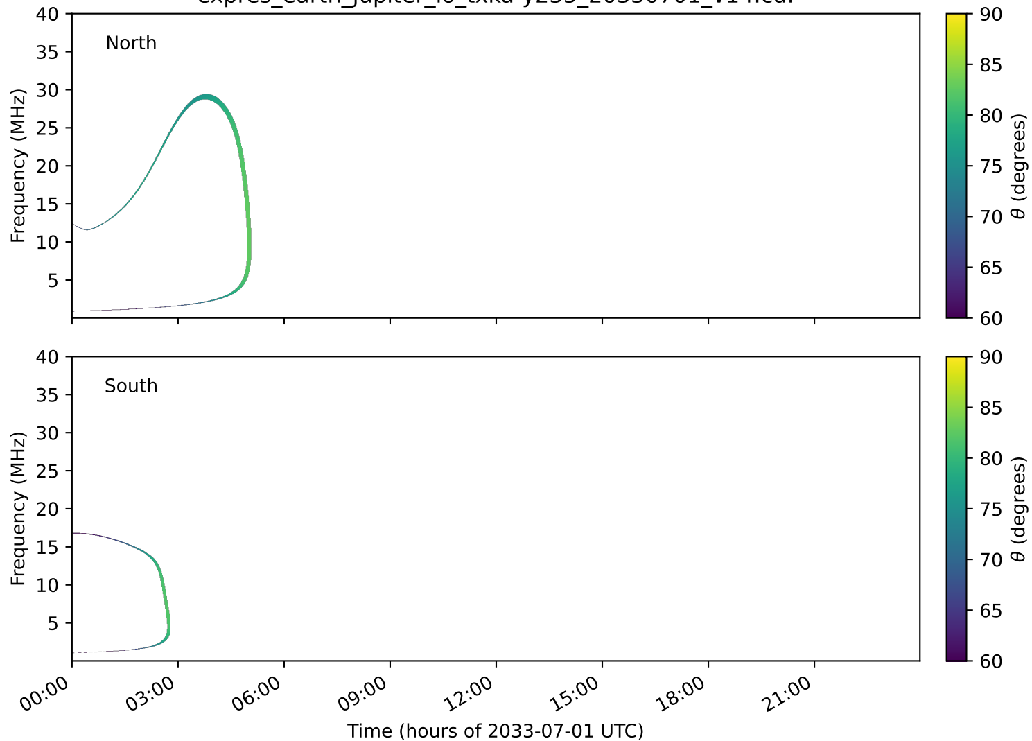
expres_earth_jupiter_io_txka-y235_20330701_v14.cdf
