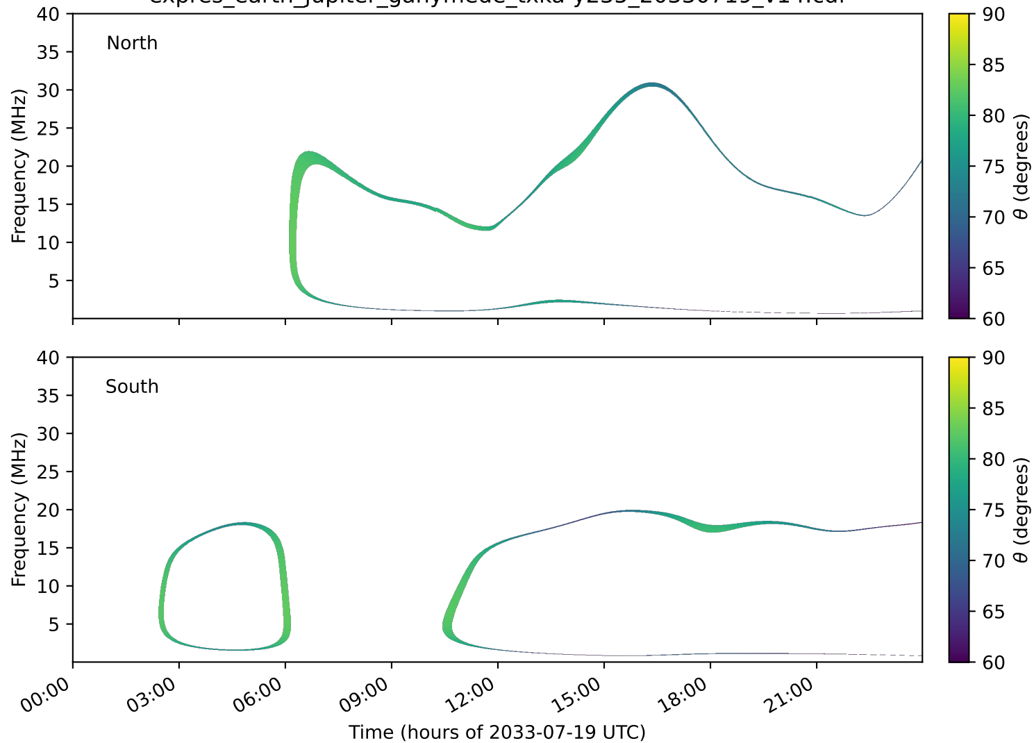
expres_earth_jupiter_ganymede_txka-y235_20330719_v14.cdf
