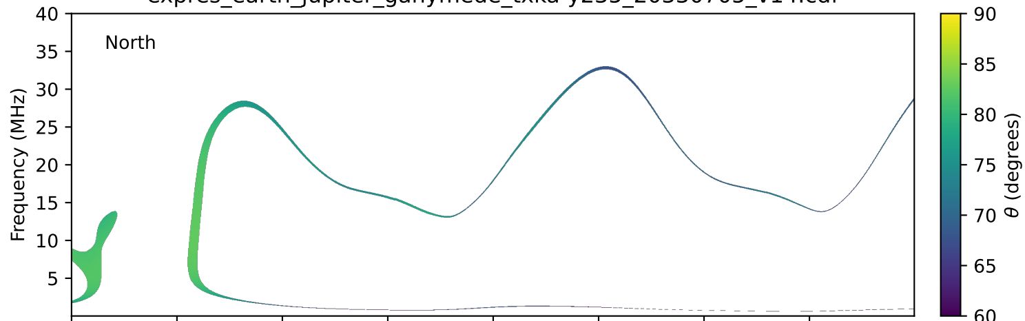
expres_earth_jupiter_ganymede_txka-y235_20330705_v14.cdf
