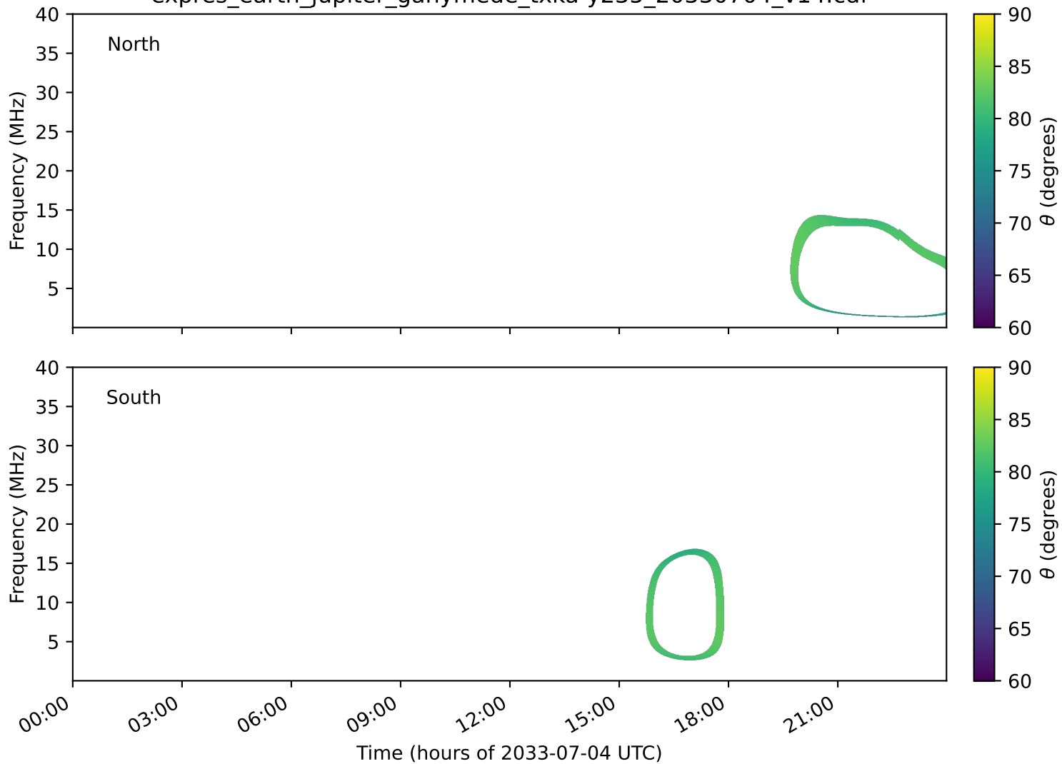
expres_earth_jupiter_ganymede_txka-y235_20330704_v14.cdf
