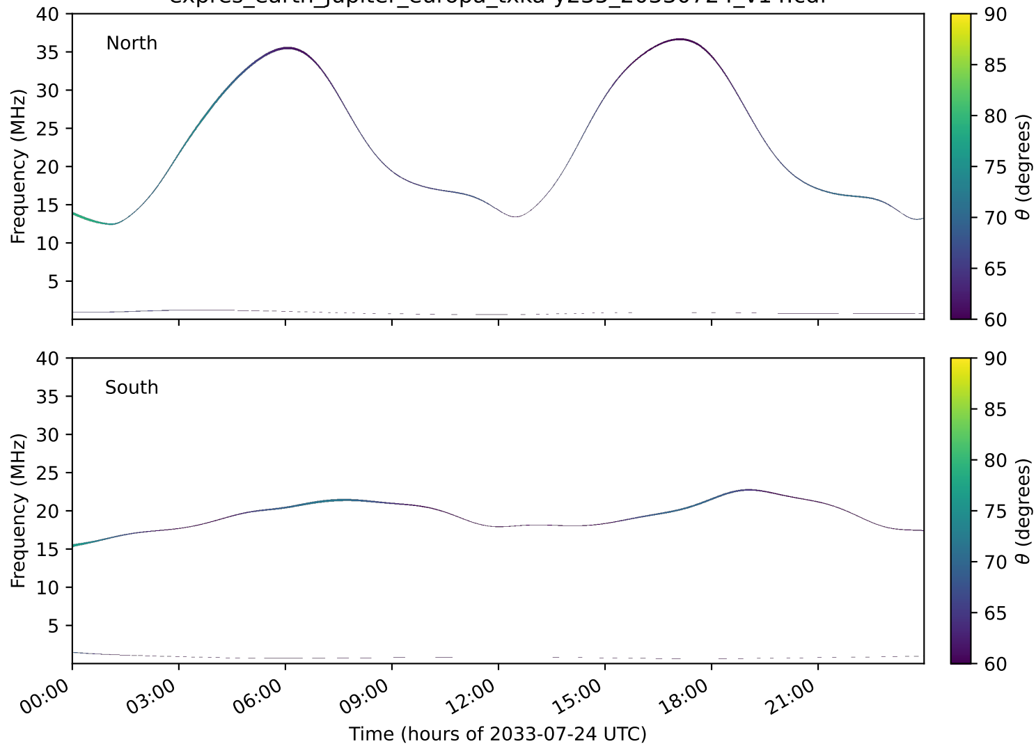
expres_earth_jupiter_europa_txka-y235_20330724_v14.cdf
