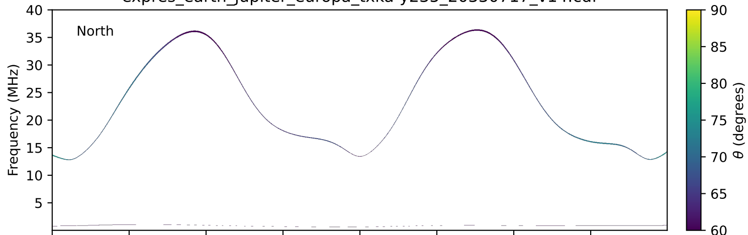
expres_earth_jupiter_europa_txka-y235_20330717_v14.cdf
