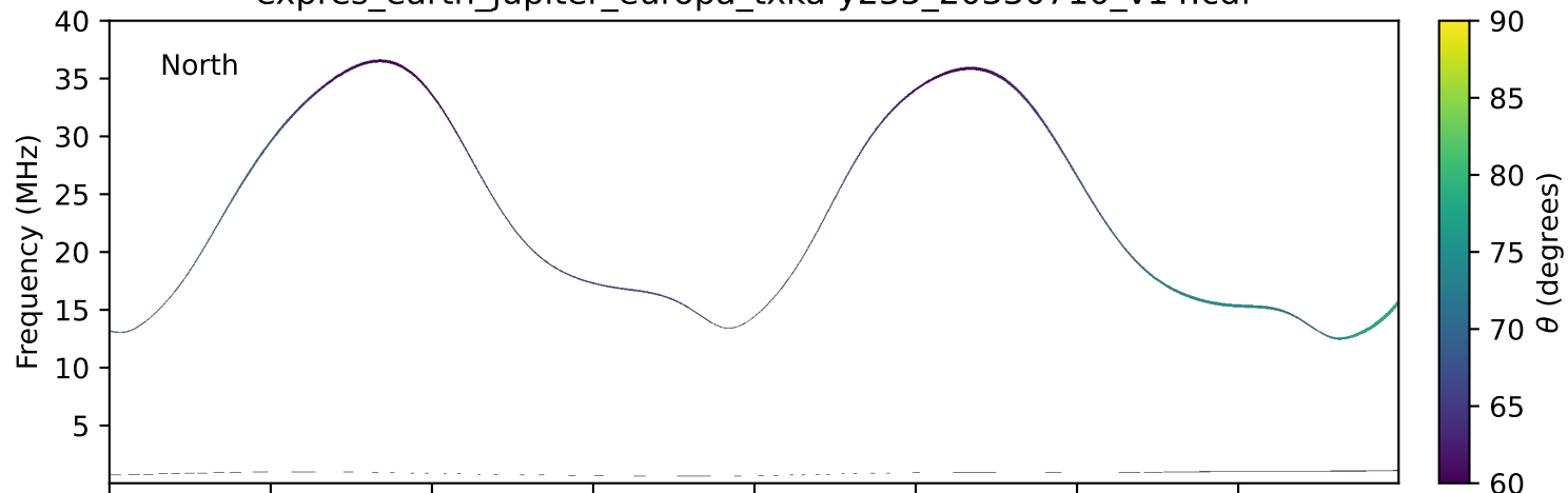
expres_earth_jupiter_europa_txka-y235_20330710_v14.cdf
