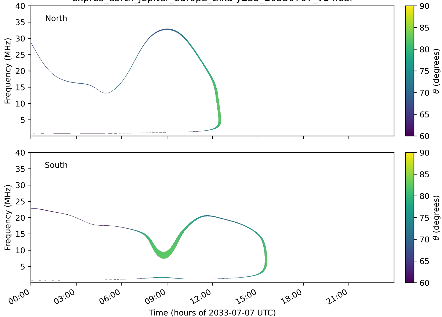
expres_earth_jupiter_europa_txka-y235_20330707_v14.cdf
