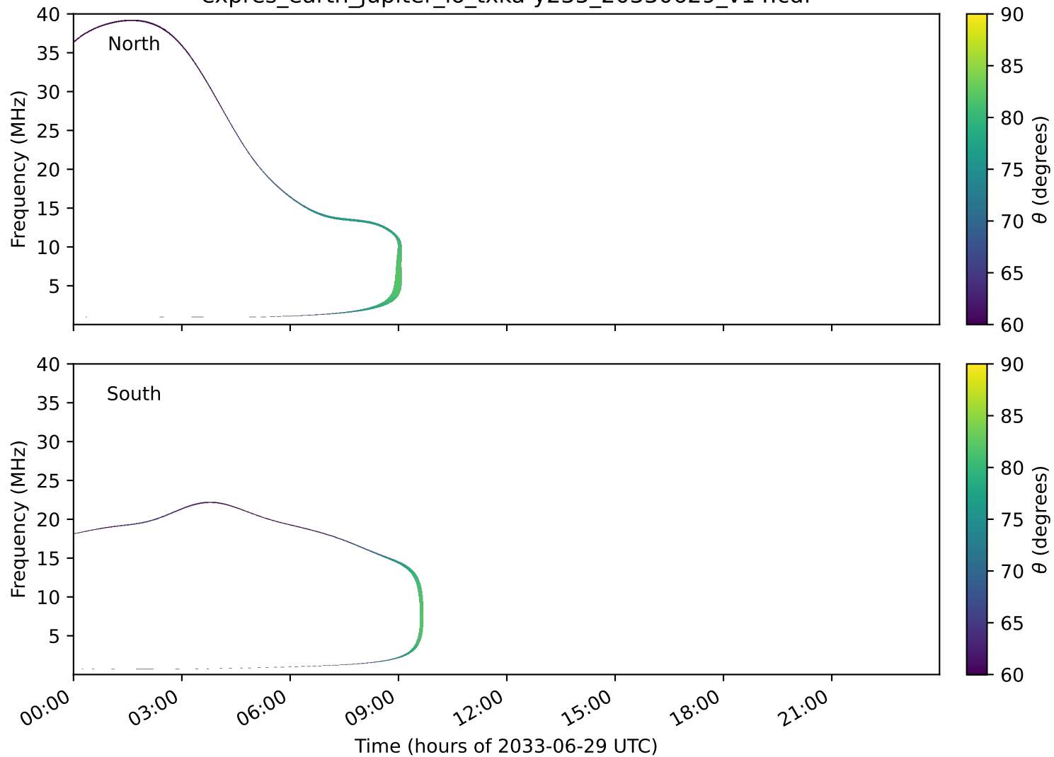
expres_earth_jupiter_io_txka-y235_20330629_v14.cdf
