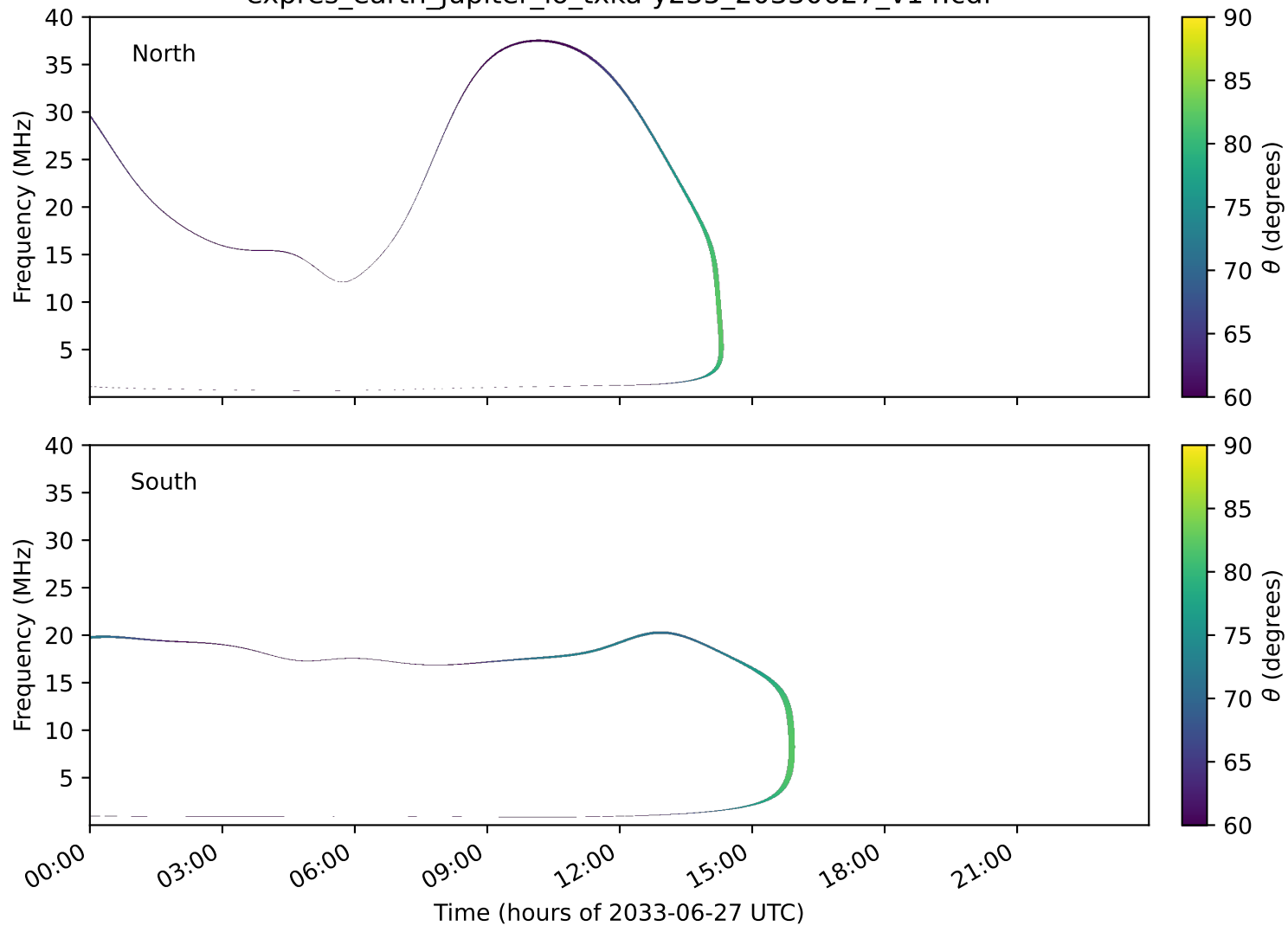
expres_earth_jupiter_io_txka-y235_20330627_v14.cdf
