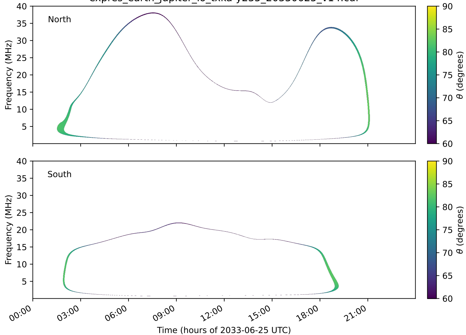
expres_earth_jupiter_io_txka-y235_20330625_v14.cdf
