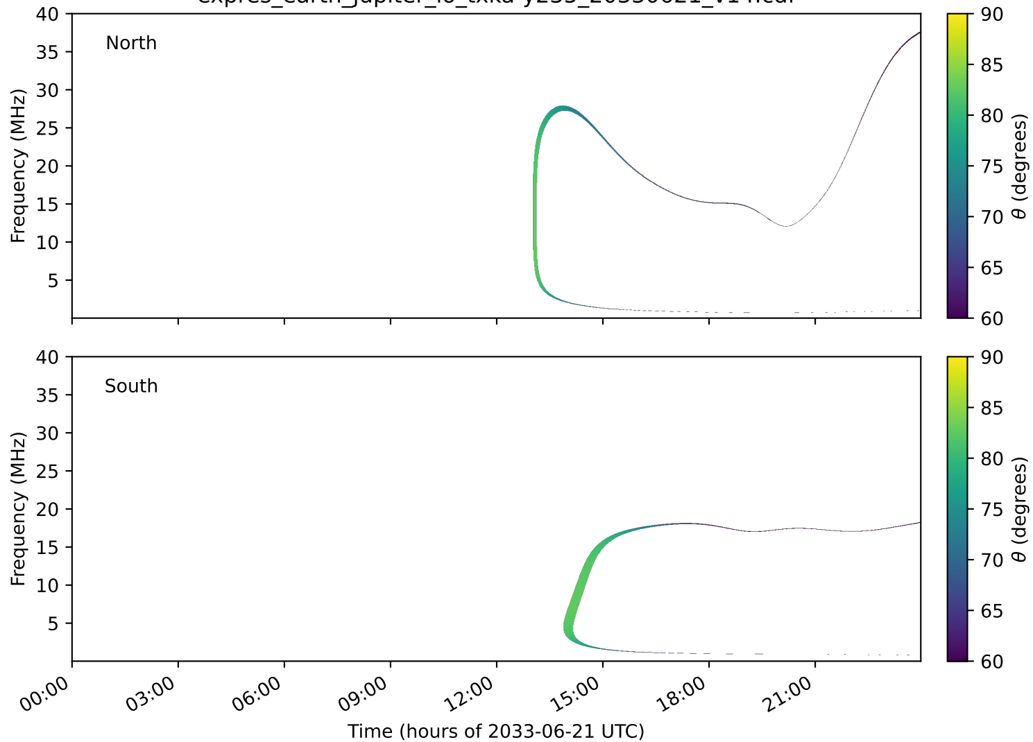
expres_earth_jupiter_io_txka-y235_20330621_v14.cdf
