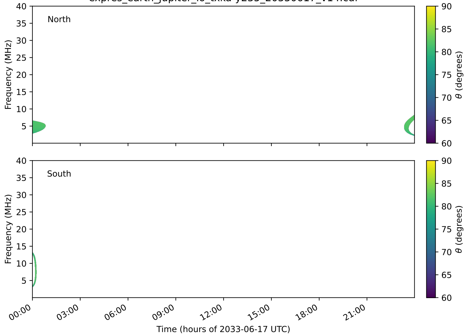
expres_earth_jupiter_io_txka-y235_20330617_v14.cdf
