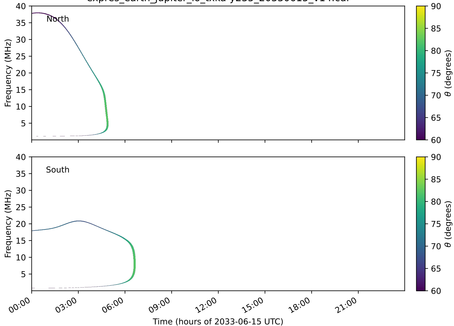
expres_earth_jupiter_io_txka-y235_20330615_v14.cdf
