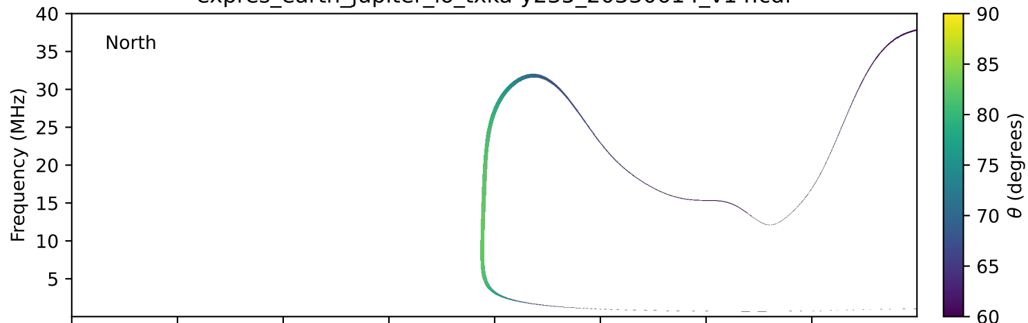
expres_earth_jupiter_io_txka-y235_20330614_v14.cdf
