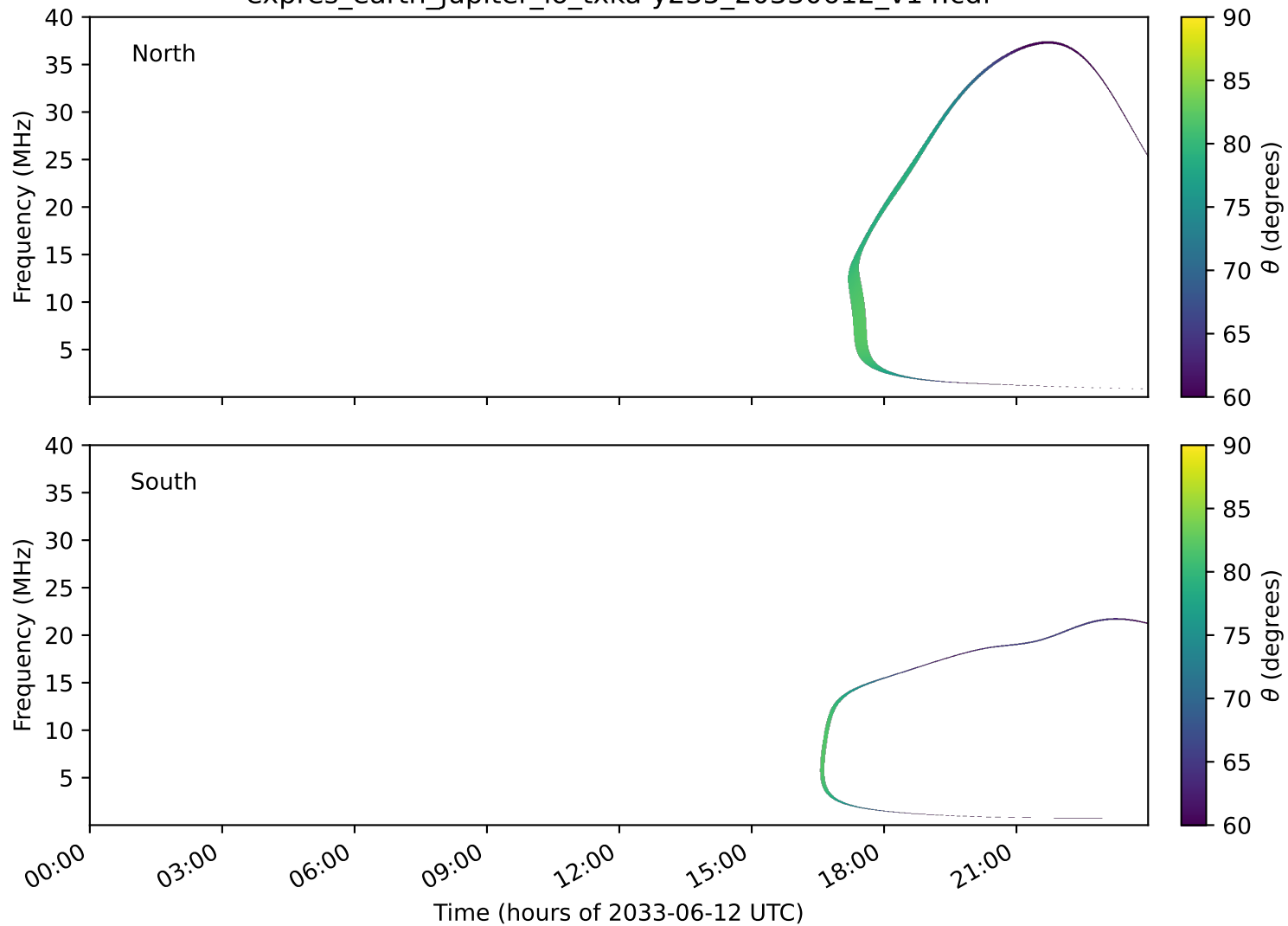
expres_earth_jupiter_io_txka-y235_20330612_v14.cdf
