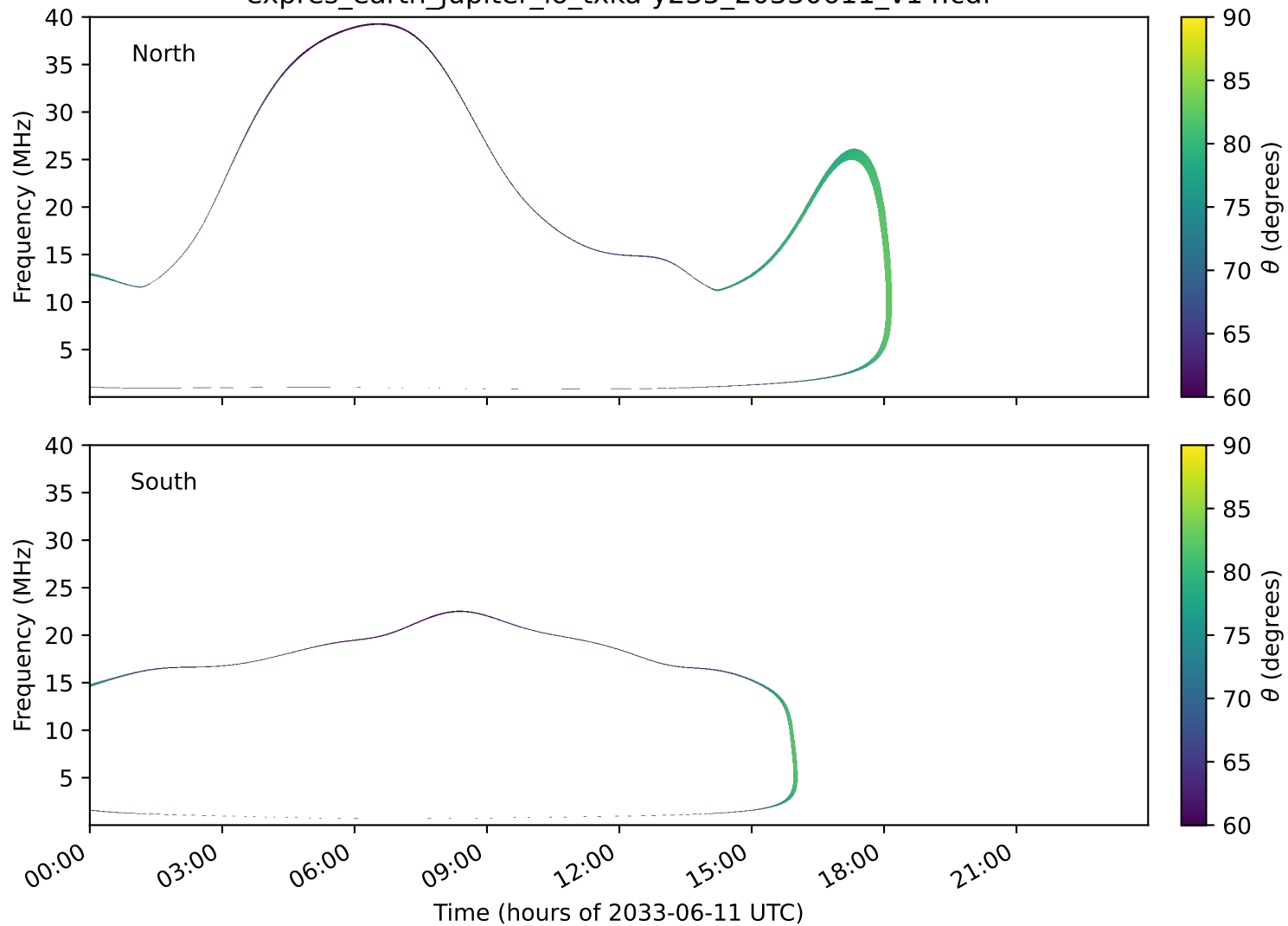
expres_earth_jupiter_io_txka-y235_20330611_v14.cdf
