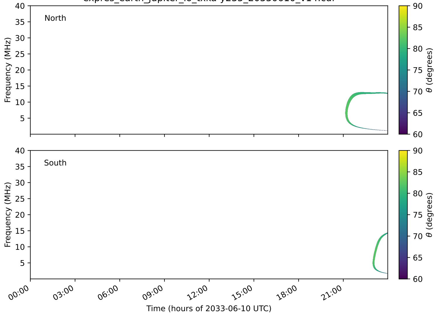
expres_earth_jupiter_io_txka-y235_20330610_v14.cdf
