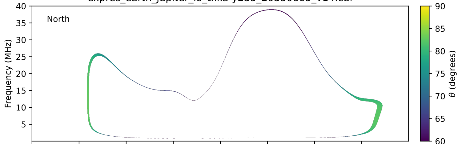
expres_earth_jupiter_io_txka-y235_20330609_v14.cdf
