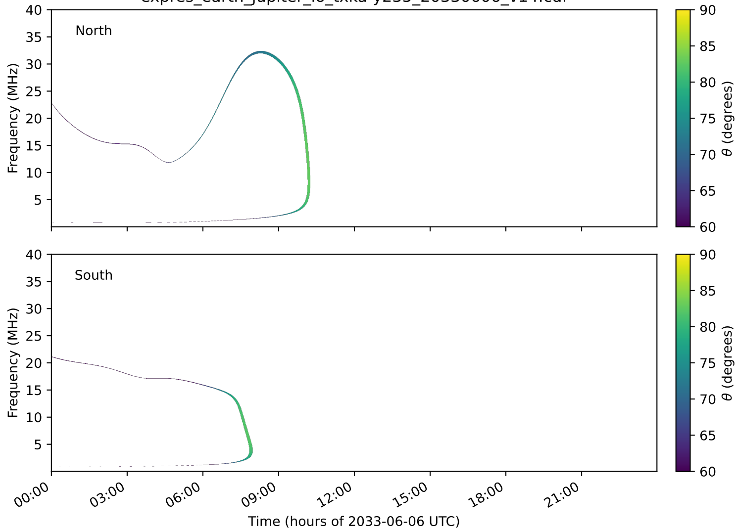
expres_earth_jupiter_io_txka-y235_20330606_v14.cdf
