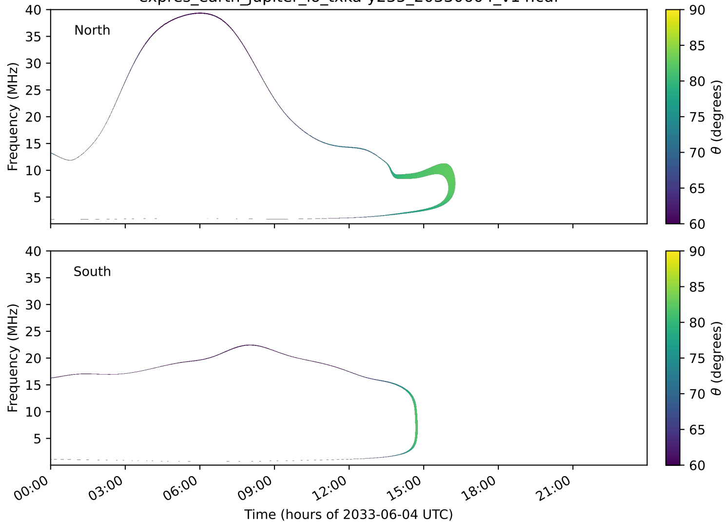
expres_earth_jupiter_io_txka-y235_20330604_v14.cdf
