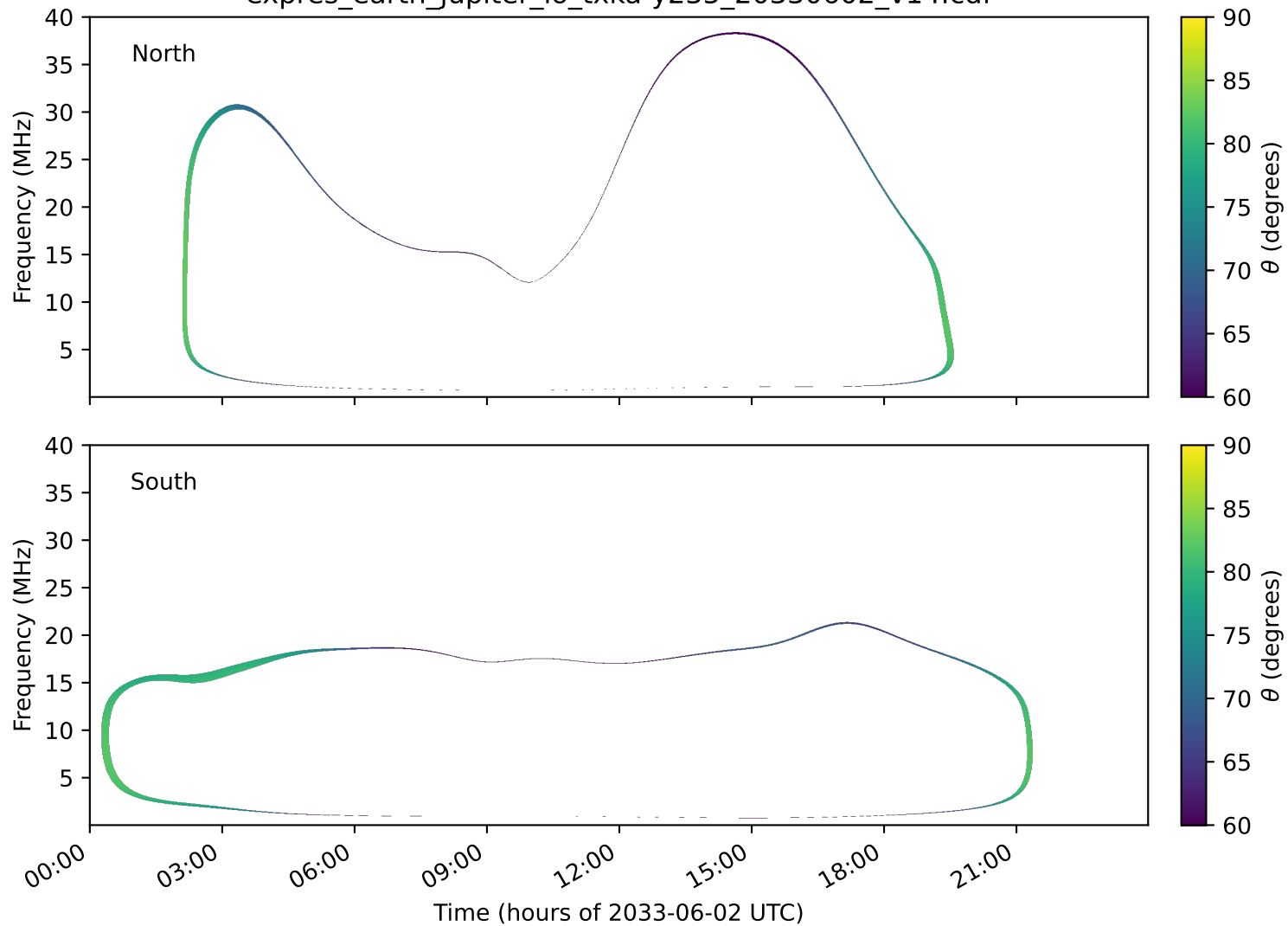
expres_earth_jupiter_io_txka-y235_20330602_v14.cdf
