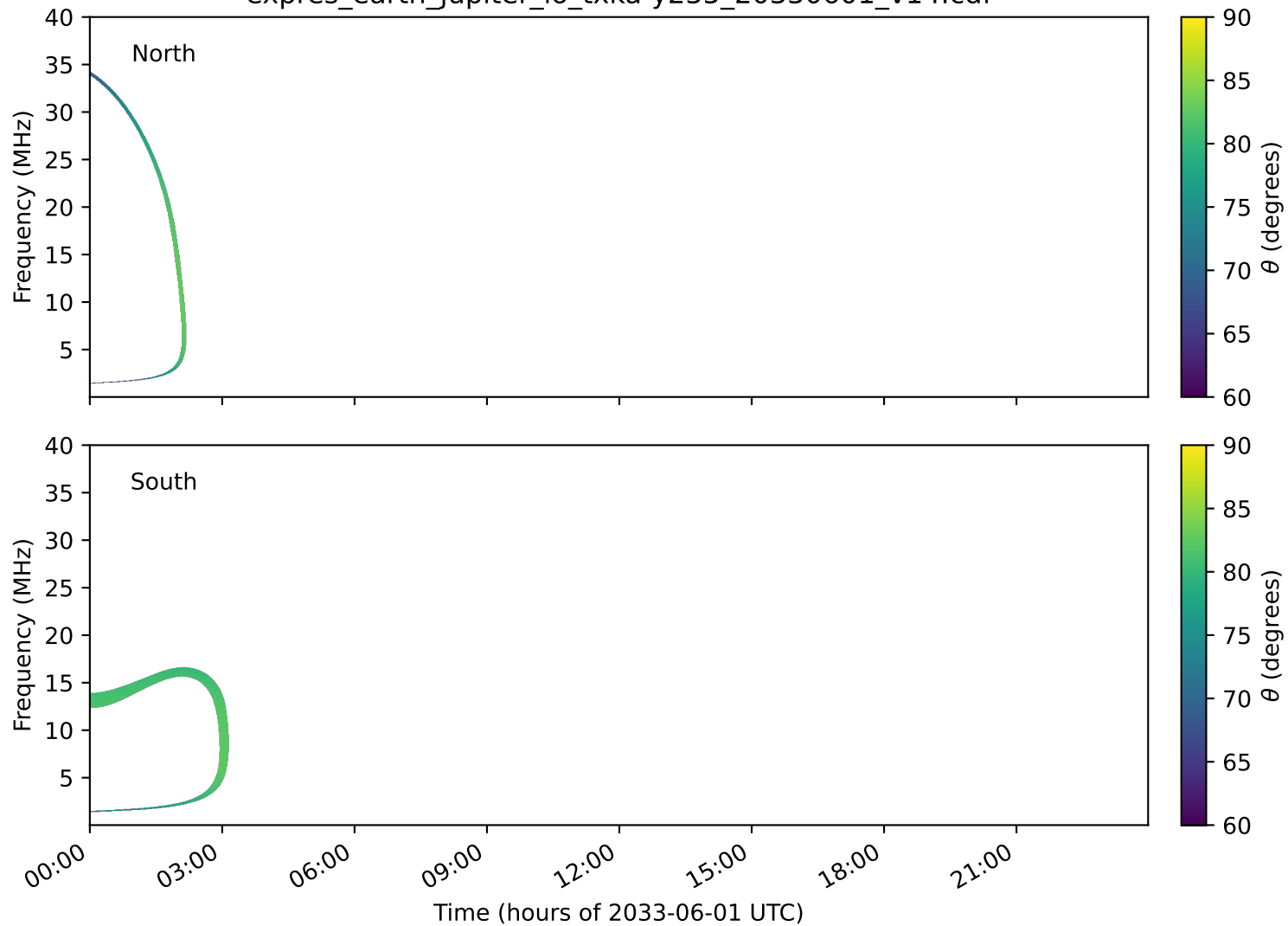
expres_earth_jupiter_io_txka-y235_20330601_v14.cdf
