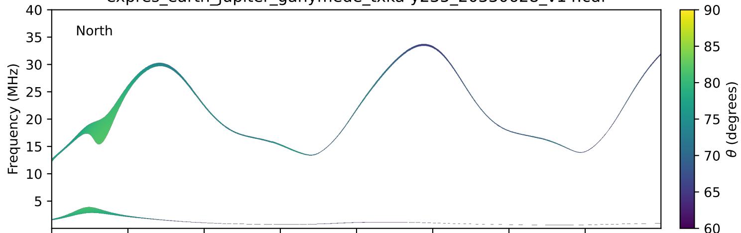
expres_earth_jupiter_ganymede_txka-y235_20330628_v14.cdf
